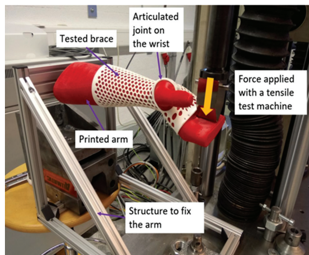
Fig. 2 (A) Test bench used to measure the brace stiffness in flexion and extension (forced wrist extension illustrated). (B) Stiffness curves for forced extension, representing the bending moment as function of the angular rotation: 3D splint with cable ties (red), lace (yellow), circular SoftCAST, split SoftCAST with bandage, and prefabricated ManuLoc splint. Reference bending moment for stiffness value determination (dashed red horizontal line).
