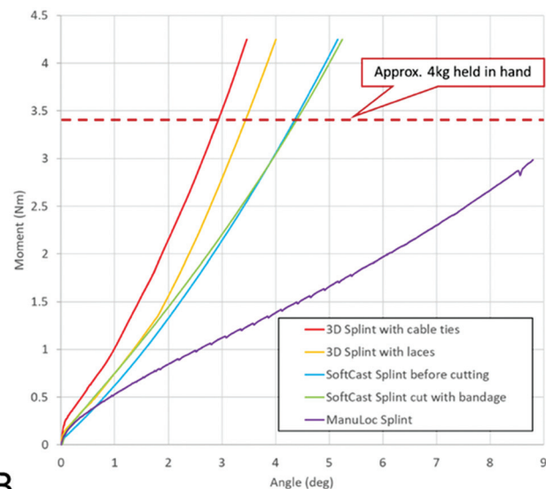
Fig. 2 (A) Test bench used to measure the brace stiffness in flexion and extension (forced wrist extension illustrated). (B) Stiffness curves for forced extension, representing the bending moment as function of the angular rotation: 3D splint with cable ties (red), lace (yellow), circular SoftCAST, split SoftCAST with bandage, and prefabricated ManuLoc splint. Reference bending moment for stiffness value determination (dashed red horizontal line).
