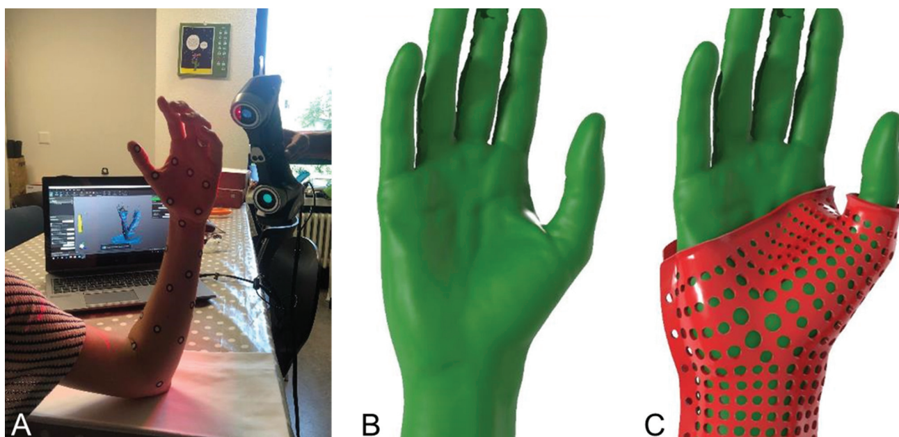
Fig. 1 Scanning procedure for a scaphoid splint. (A) Scanning the forearm with HandySCAN 300, reflecting self-adhesive dots are positioned on the arm to increase scanning quality. (B) Virtual forearm model. (C) Patient-specific anatomical brace model ready to be printed.
